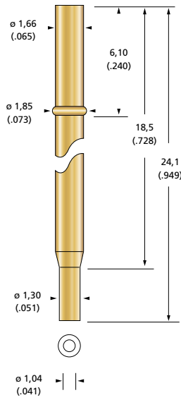
S 21.00-C Open Crimp End
