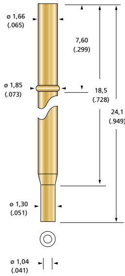
S 21.01-C Open Crimp End
