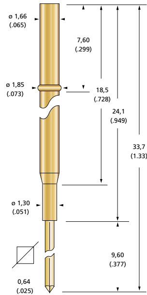
S 21.01-W Wire-Wrap-Post
